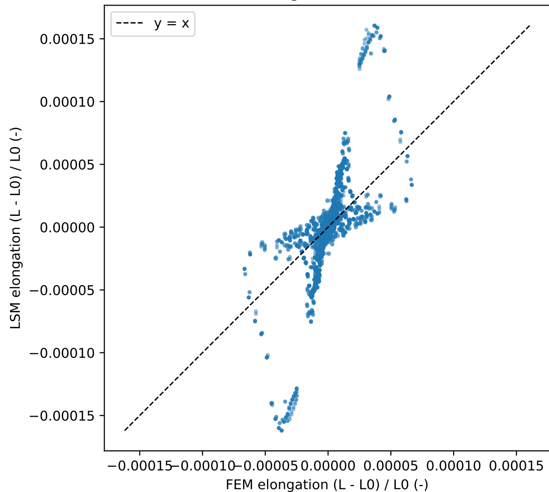
Bond elongation: LSM vs FEM
