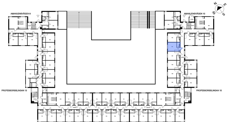
Planritning/Floor plan
