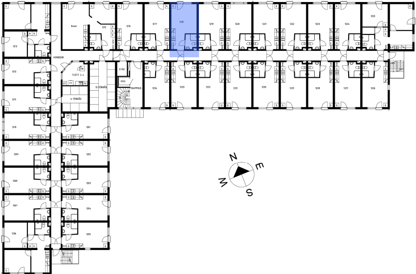
Planritning/Floor plan
