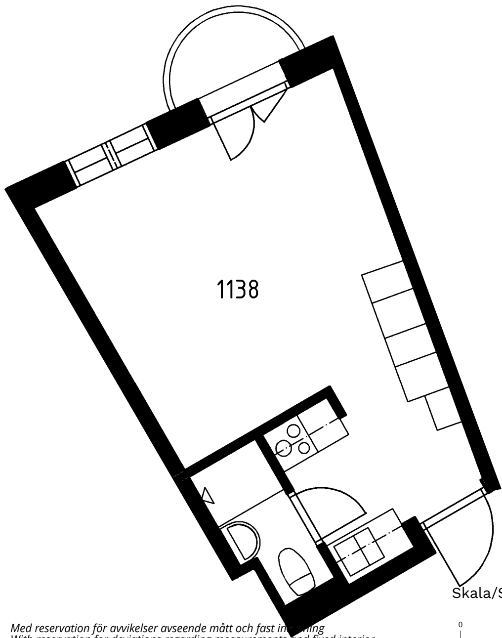
Planritning/Floor plan
