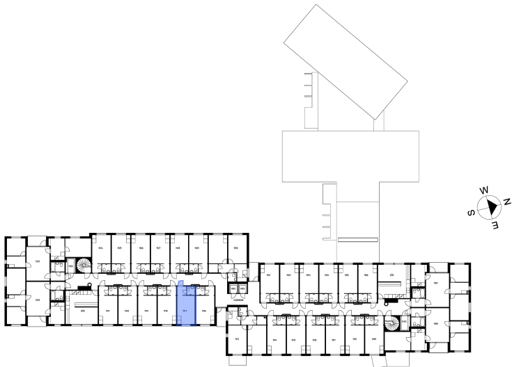
Planritning/Floor plan
