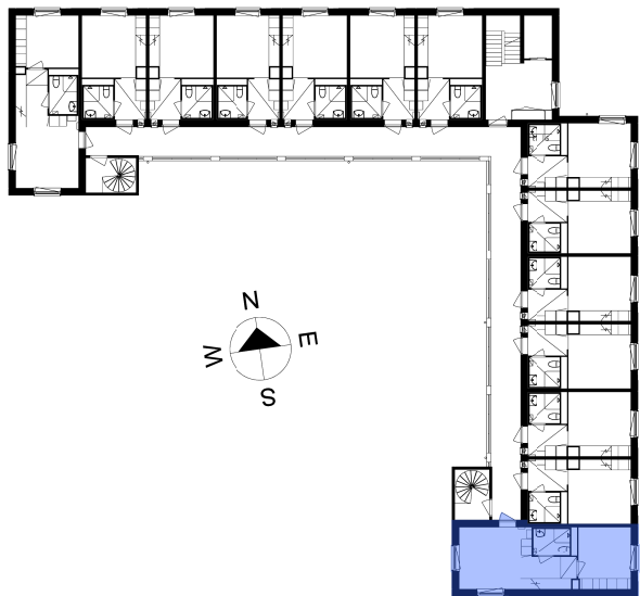
Planritning/Floor plan
