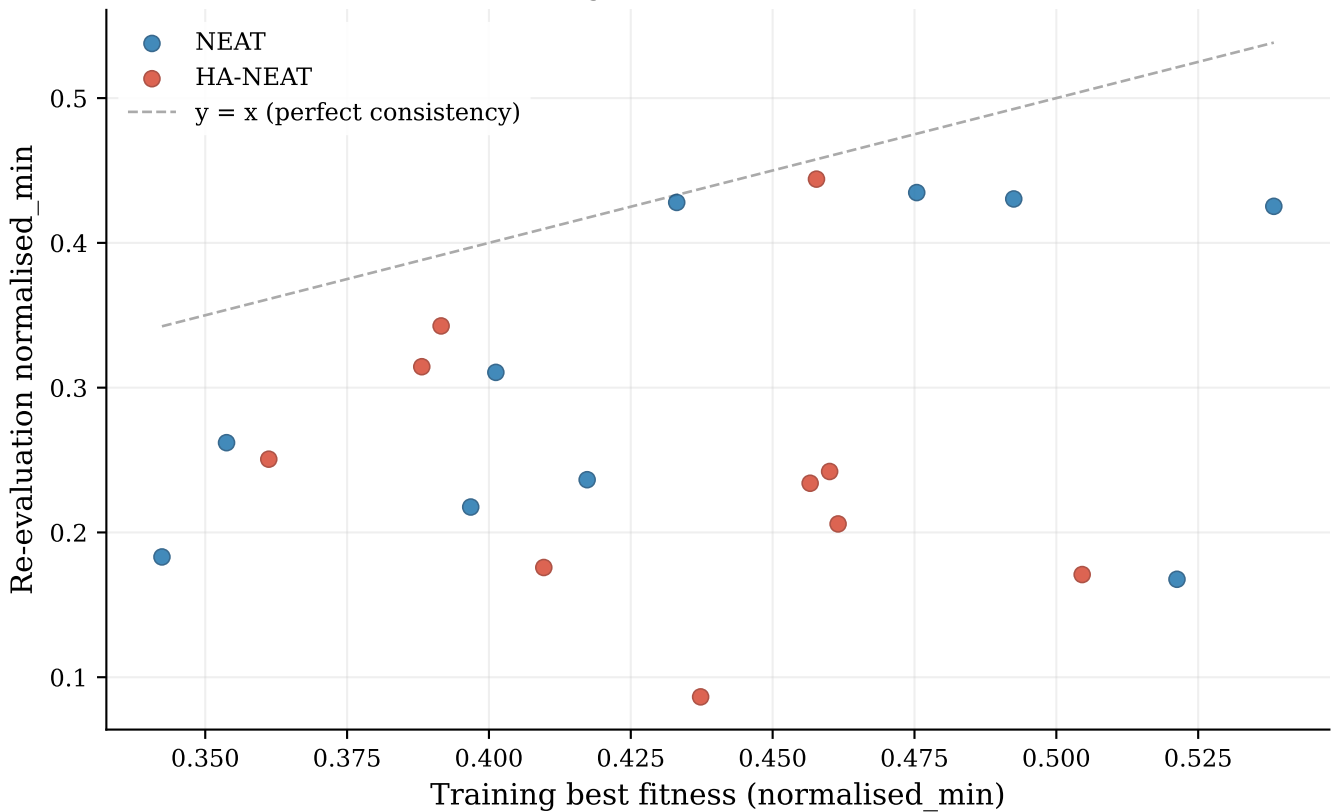
Training vs re-evaluation fitness
