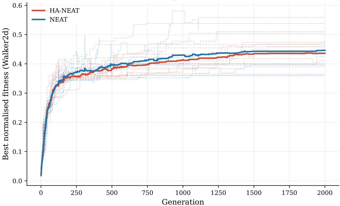
Training - Walker2d
