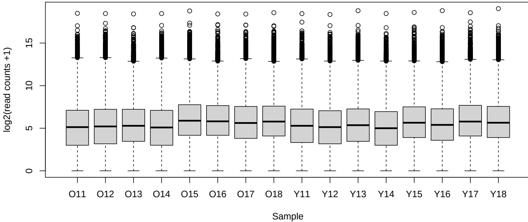
Before normalization
