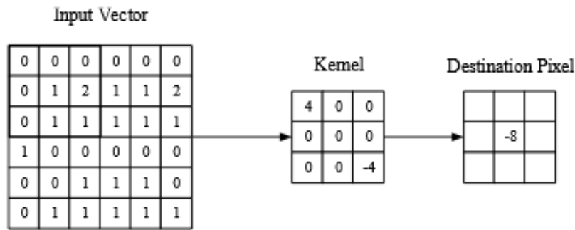
Abb. 5.3: Convolutional [39, S. 6]
