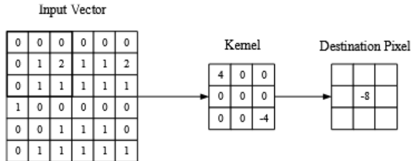
Abb. 5.3: Convolutional [26, S. 6]
