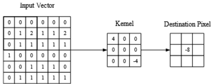
Abb. 5.3: Convolutional [24, S. 6]
