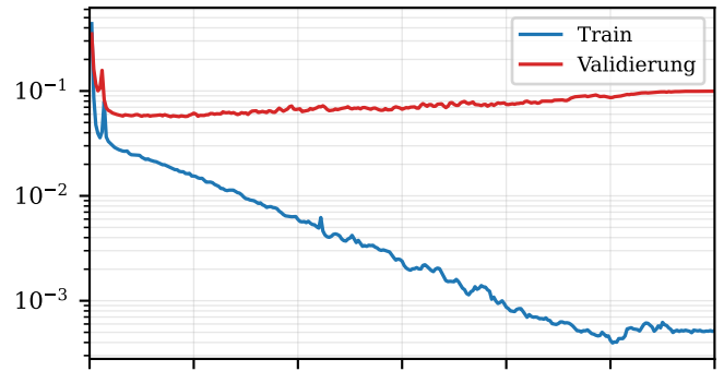
Noise-Prediction
