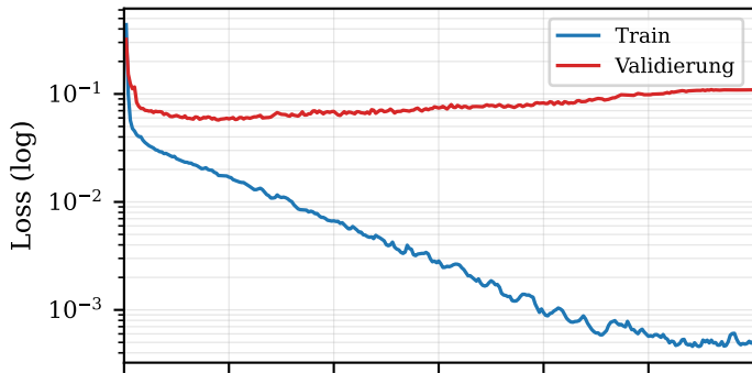
Data Augmentation
