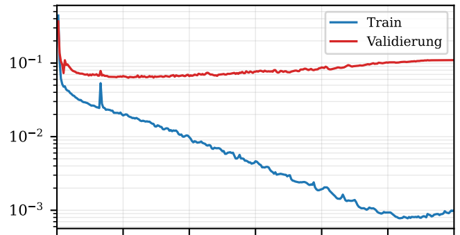
Linearer Schedule
