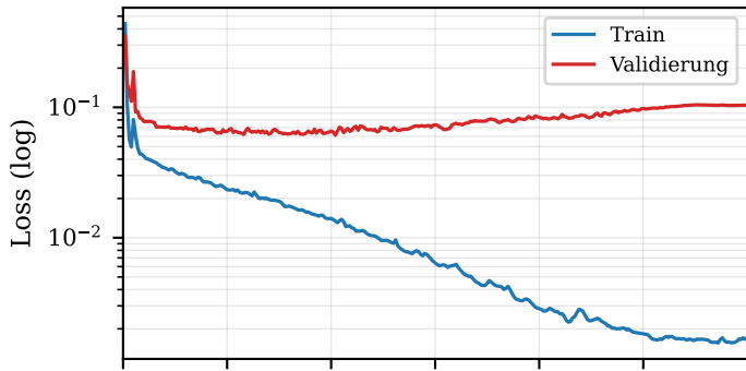
Ohne Self-Attention
