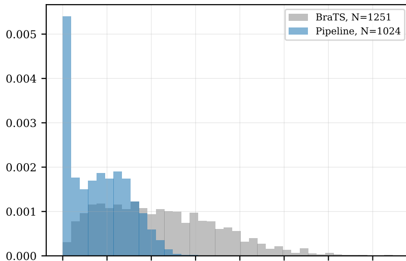
DPM-Solver++ (25)
