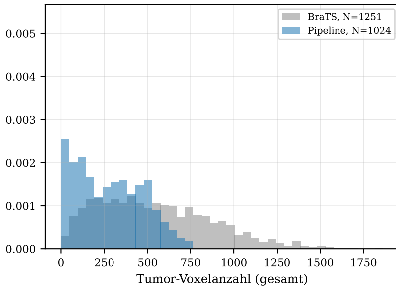
DPM-Solver++ (25)
