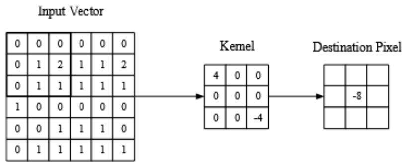
Abb. 5.3: Convolutional [46, S. 6]
