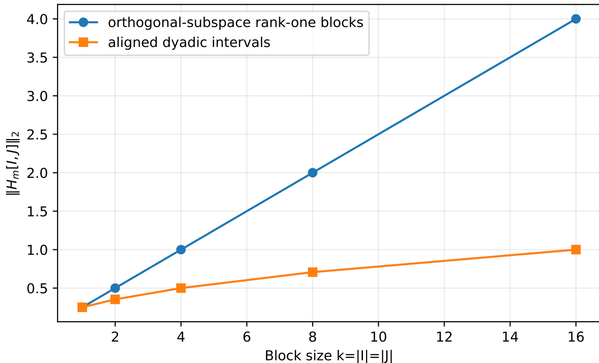
Partial Walsh norms for two structured geometries (m=16)
