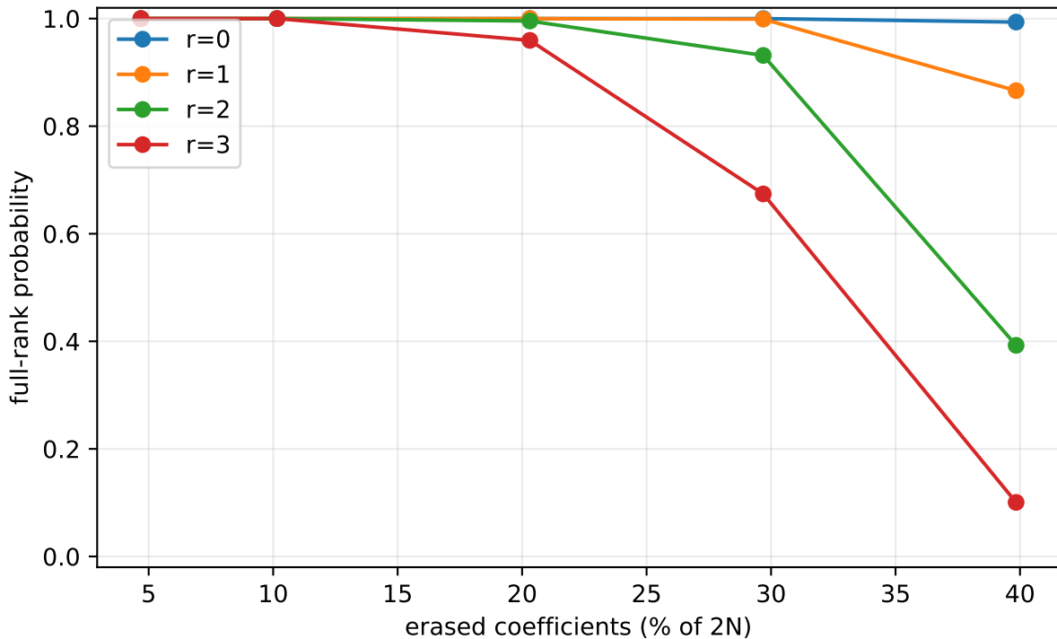
Random-erasure rank survival, N=64 , 2000 trials
