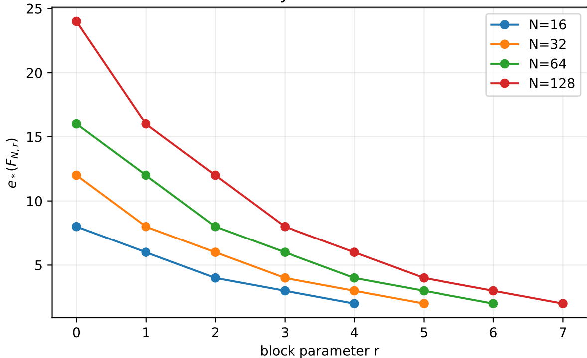
Exact locality-robustness trade-off
