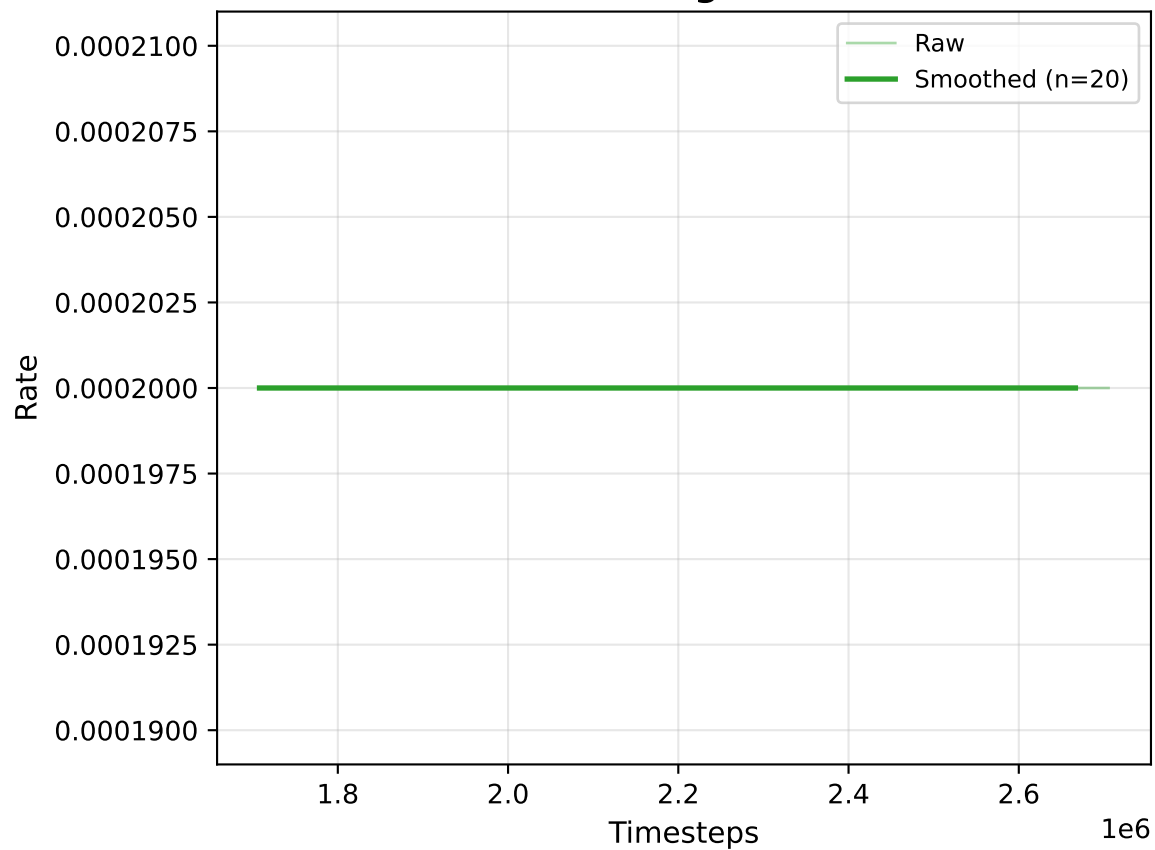
Learning Rate
