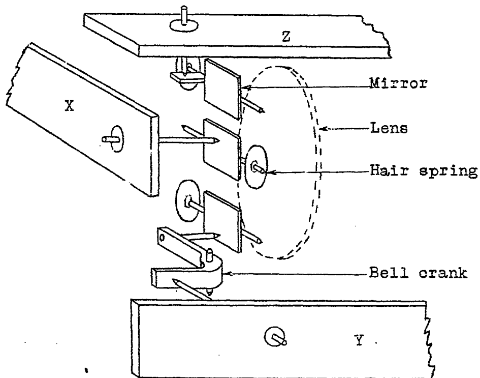
Fig. 2. Showing the means for transferring the motion of the springs to the three mirrors. The dash pots are omitted.
