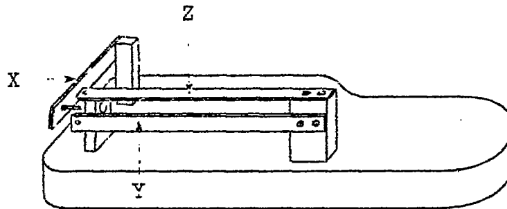
Fig. 1. Showing the arrangement of the springs and the axes of the instrument.
