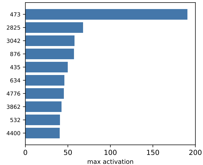
mid.0 top-10 (idx of 5120)
