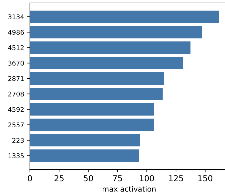
up.0.0 top-10 (idx of 5120)
