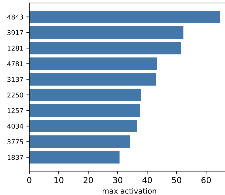
down.2.1 top-10 (idx of 5120)
