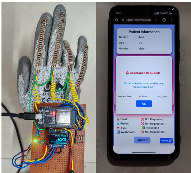
Fig 5: Flex Sensor 3 Bend Detected and Assistance Request Displayed on Mobile app
