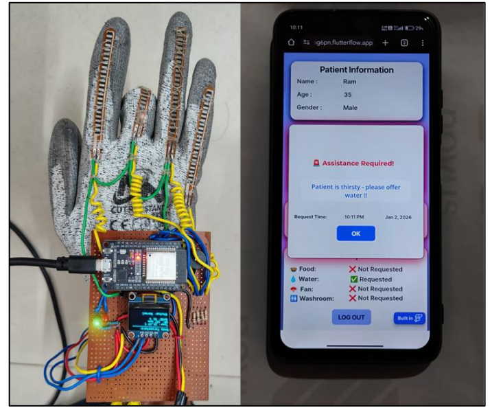
Fig 4: Flex Sensor 2 Bend Detected and Assistance Request Displayed on Mobile app
