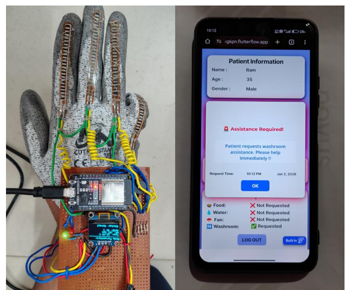
Fig 6: Flex Sensor 4 Bend Detected and Assistance Request Displayed on Mobile app
