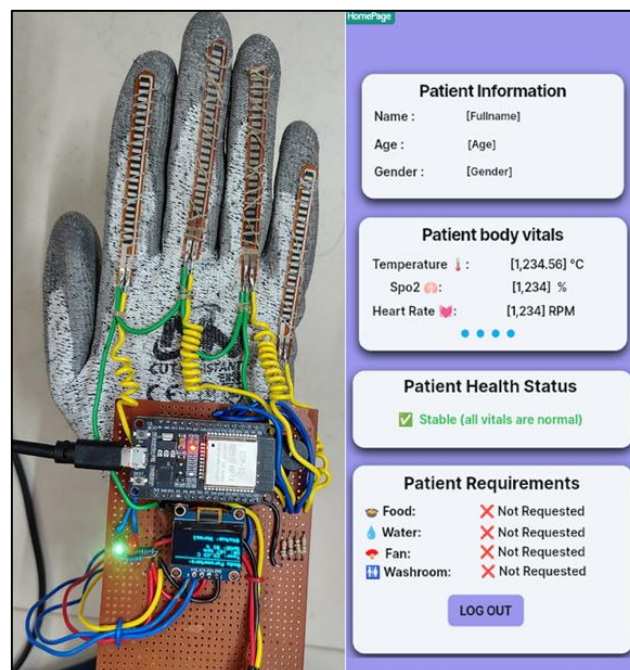
Fig 2: Hardware Integration
