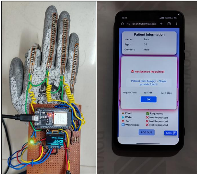
Fig 3: Flex Sensor 1 Bend Detected and Assistance Request Displayed on Mobile app
