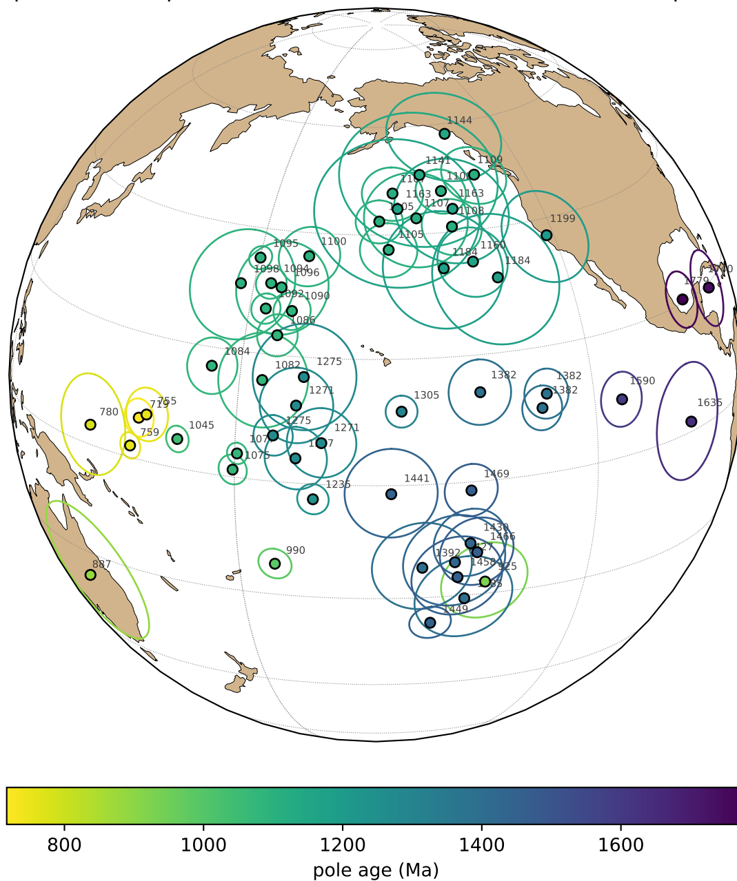
Laurentia apparent polar wander path, 1779-717 Ma (recreated-from-site-level poles; Greenland rotated)
