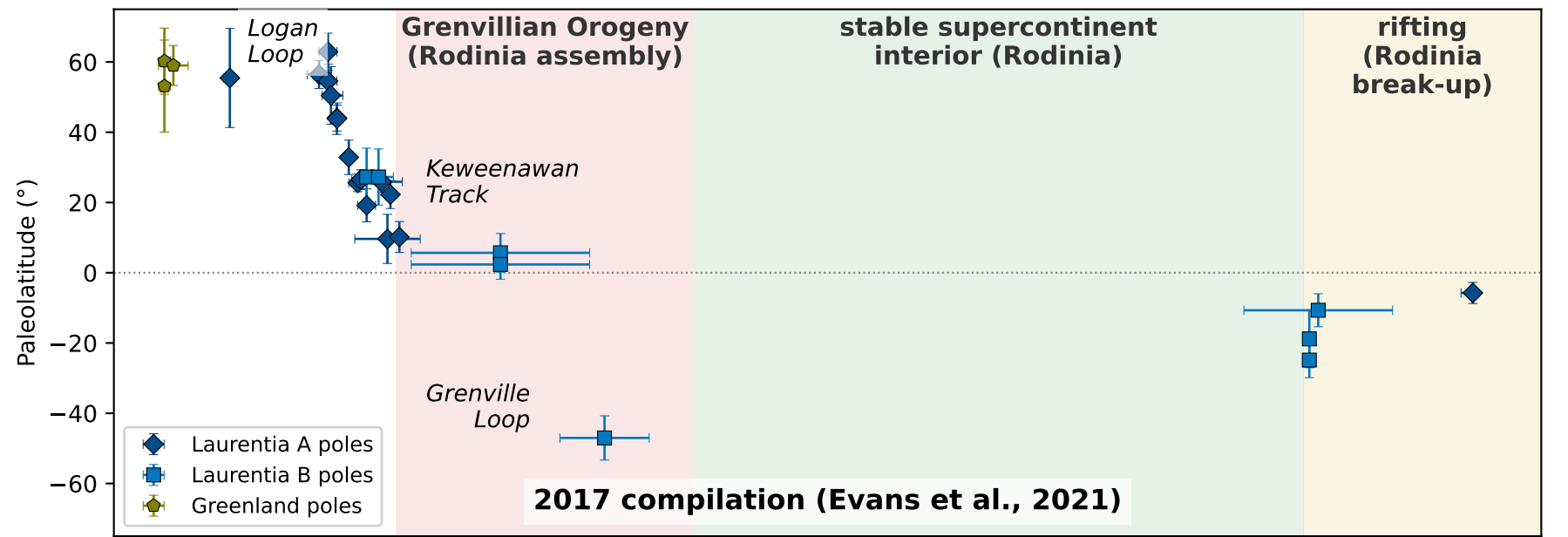
Position of Duluth (lat = 46.79°N, lon = 92.10°W) implied by Laurentia poles
