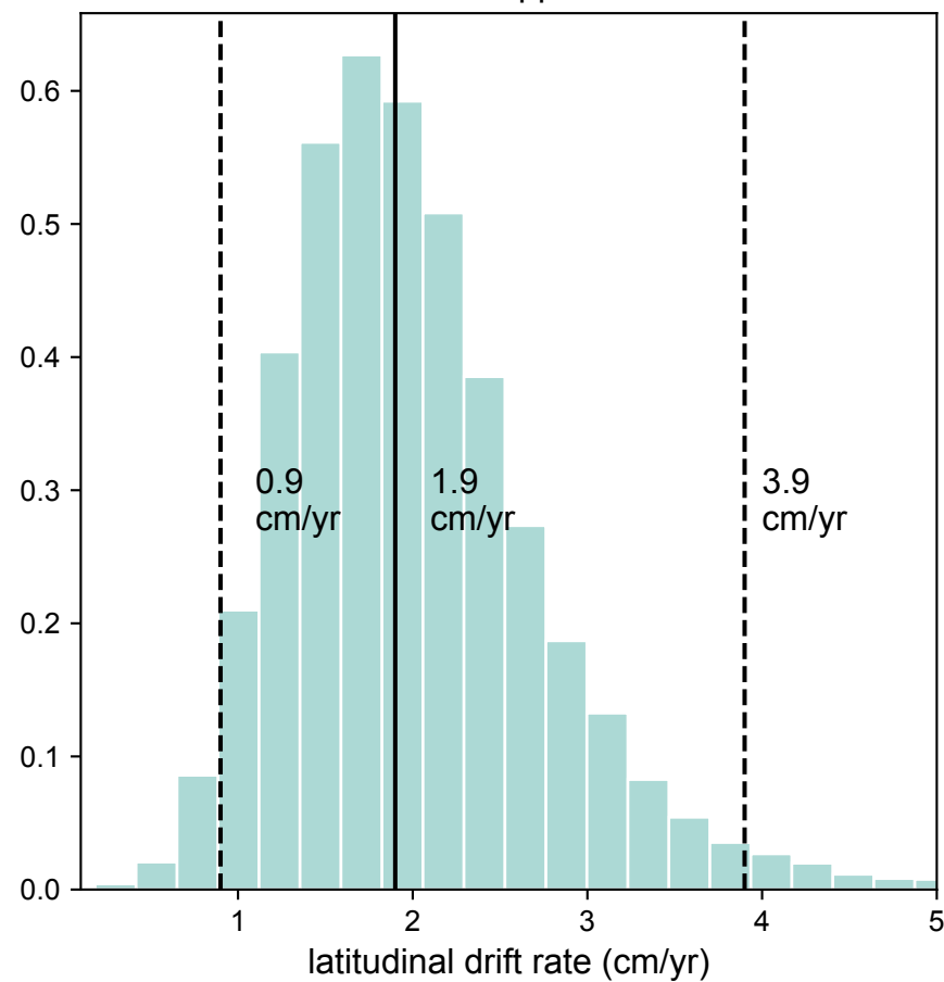
Lower Freda to Upper Freda Pole
