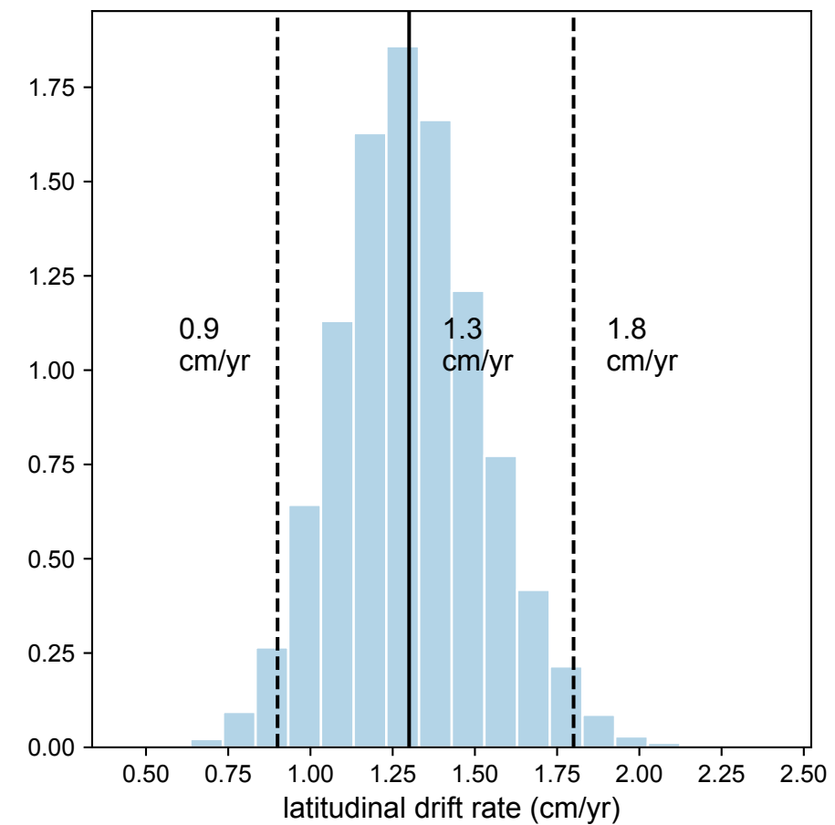
Lower Freda to Jacobsville Pole
