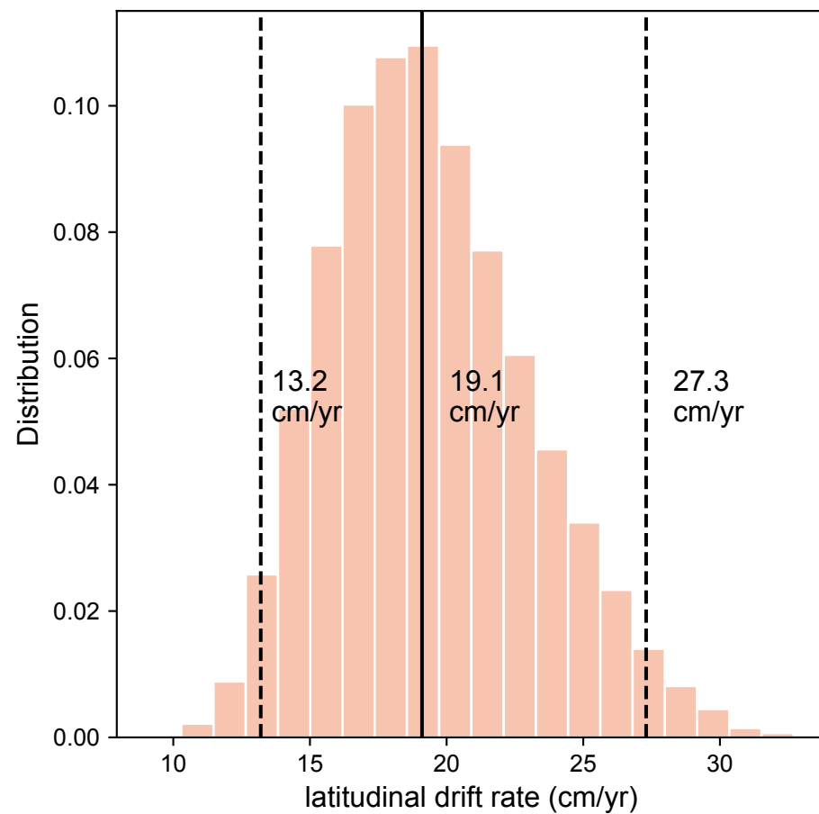
Lower Osler Pole to Lower Freda Pole
