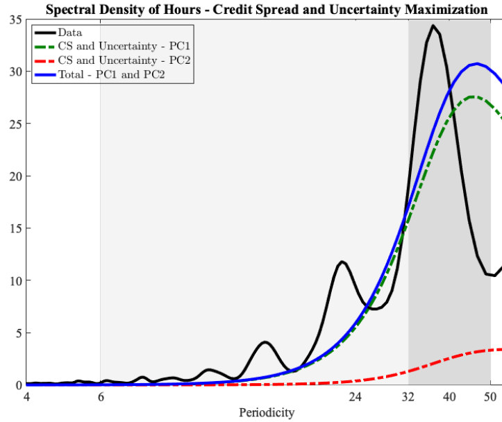
Figure 5: Hours Spectrum under the Joint Rotation Notes. The black line is the spectral density of hours in the data. The green and red dashed lines are the spectra attributable to the first and second principal components of the joint credit-spread and uncertainty objective. The blue line is their sum. The shaded region marks periodicities from 32 to 50 quarters.
