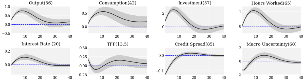
Figure 4: Impulse Responses to the Joint Uncertainty–Credit-Spread Shock Notes. Solid lines are posterior median responses and shaded regions are posterior credible bands. The shock jointly maximizes the normalized variance shares of the credit spread and macro uncertainty over periodicities from 6 to 40 quarters. Numbers in parentheses report variance shares over that band. The horizontal axis is in quarters.
