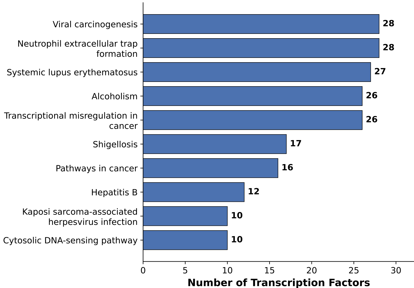
Disease Pathway
