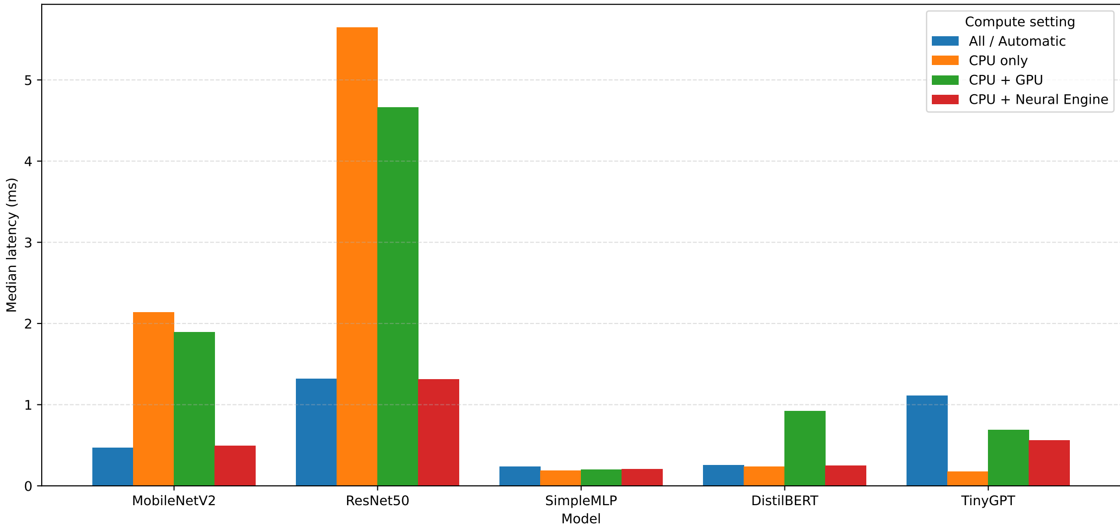
Core ML FP16 Median Latency by Model and Compute Setting
