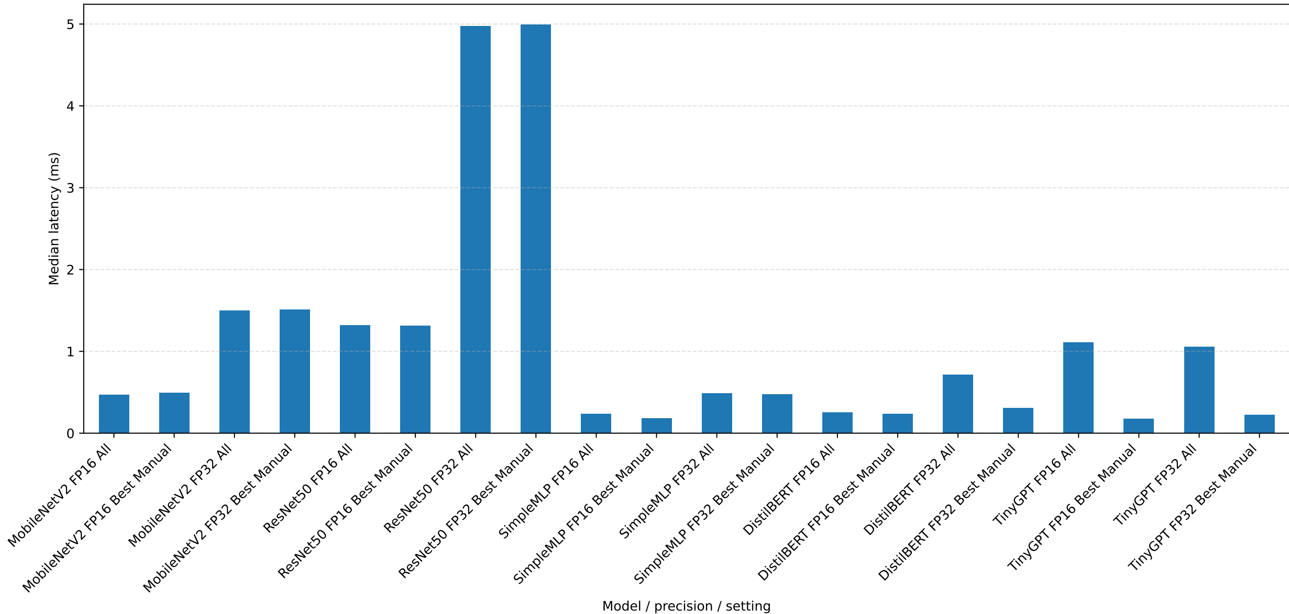
Precision Ablation: Automatic vs Best Manual Compute Setting
