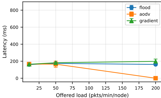
Latency P50
