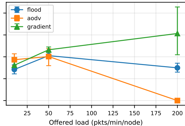
Latency P95
