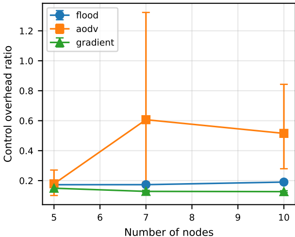
Control overhead vs network size (mixed, obs=10dB, load=50)
