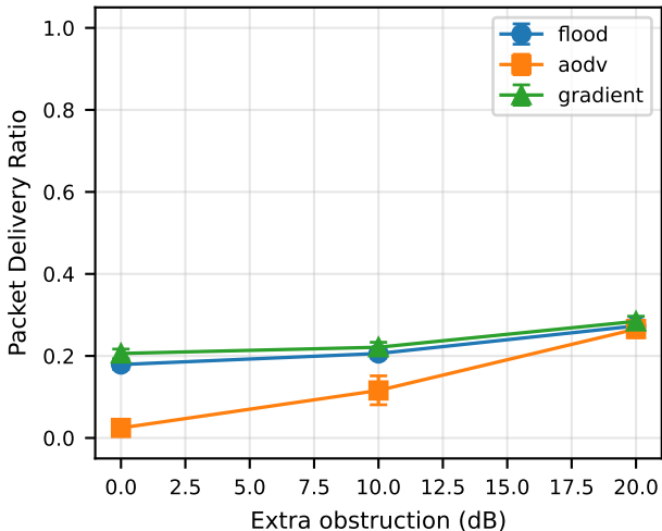
PDR vs obstruction (n=7, mixed, mob=1.0m/s, load=50)
