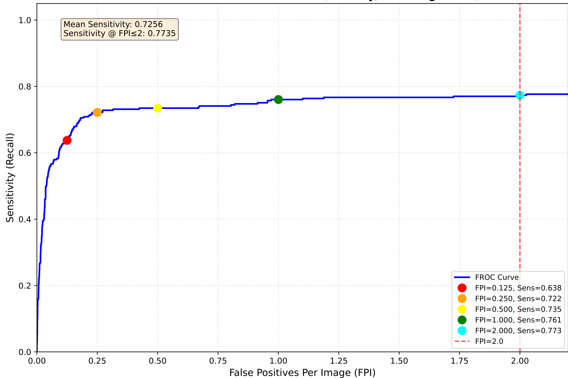
FROC Curve - DINO on TBX11K (TB-only, Class-agnostic)
