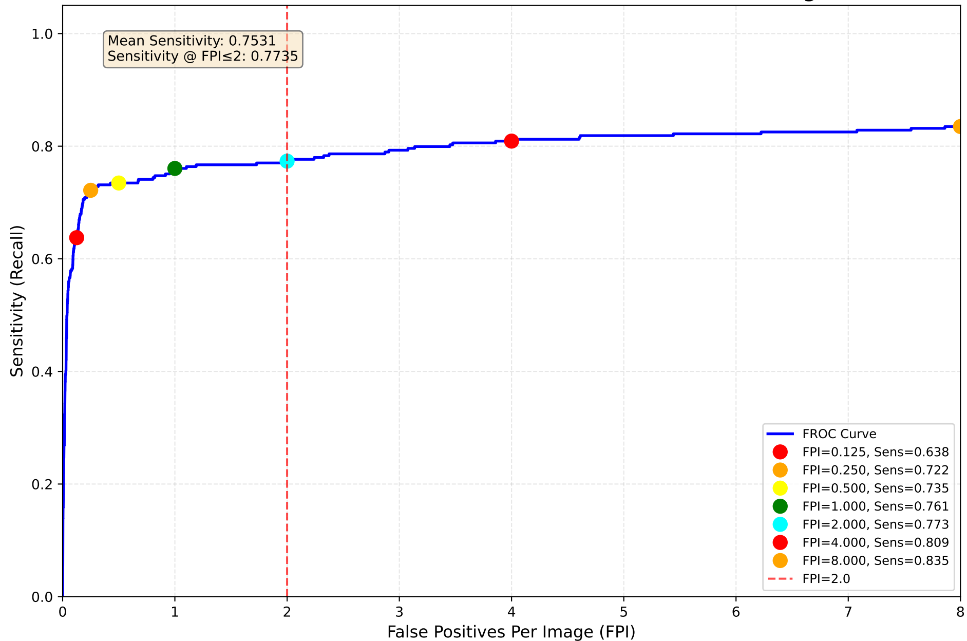
FROC Curve - Previous Evaluation (All 1800 Validation Images)
