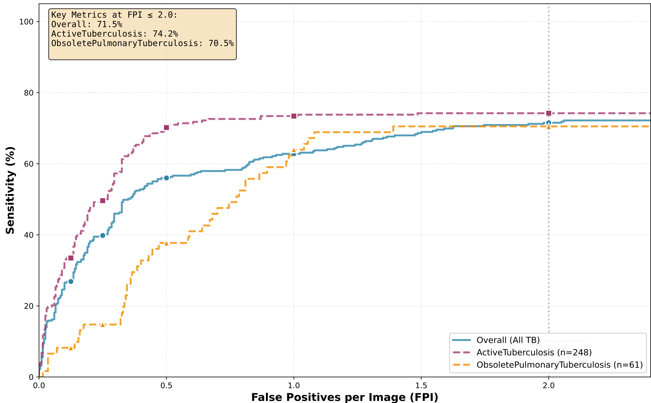
Per-Category FROC Curves: TB Detection Performance
