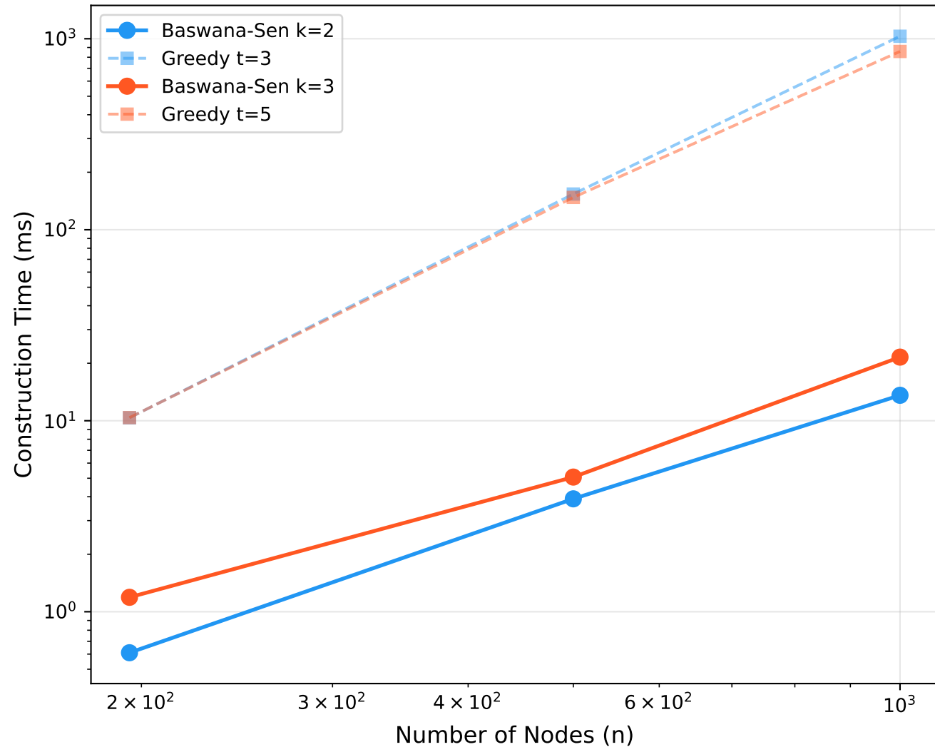
Spanner Construction Time vs Graph Size
