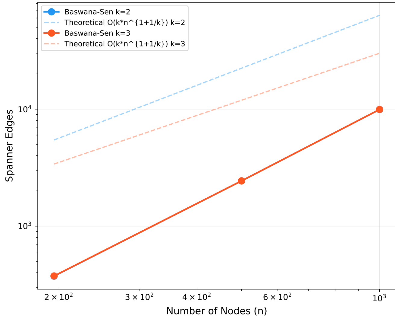
Spanner Size vs Graph Size
