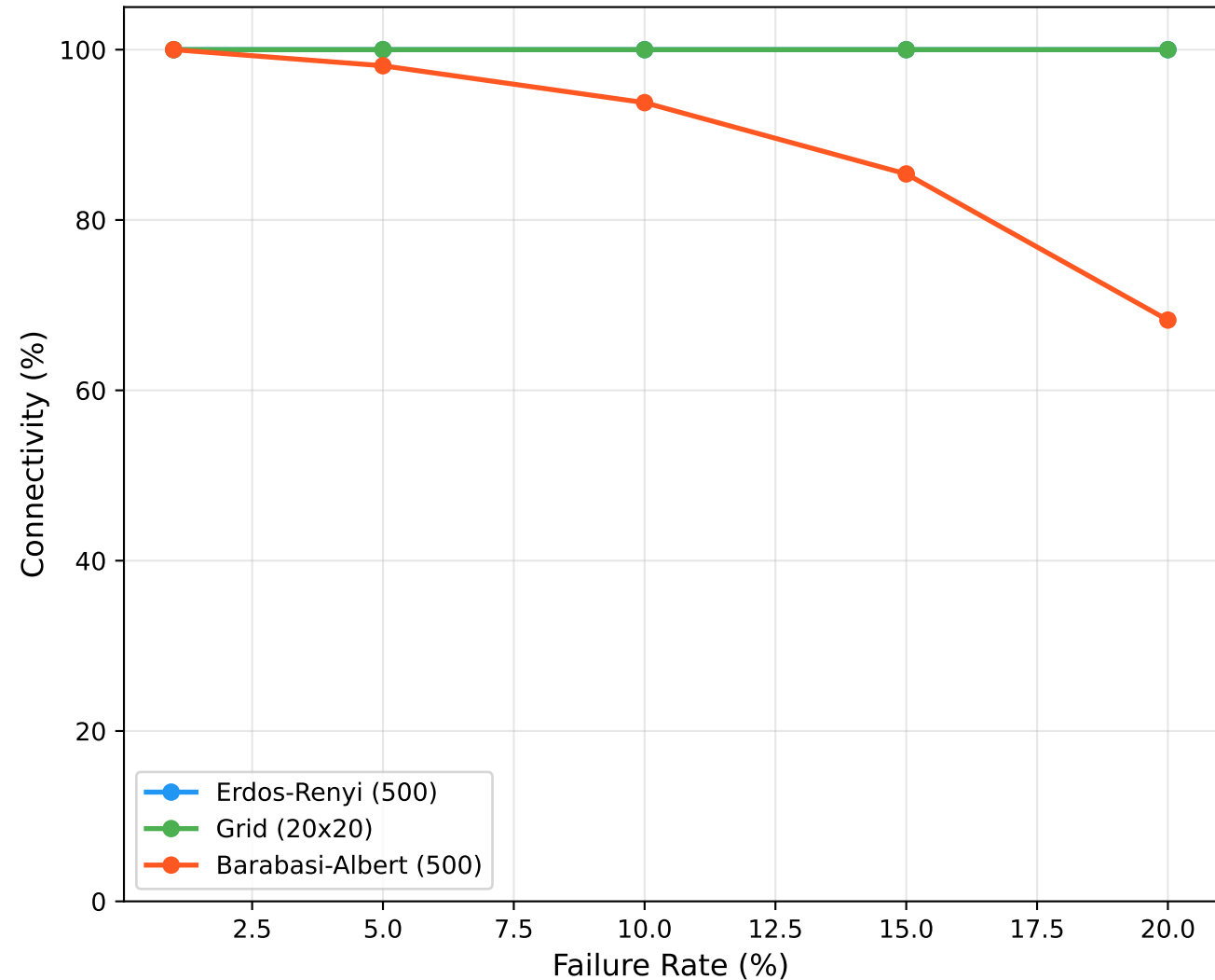
Spanner Connectivity Under Node Failures
