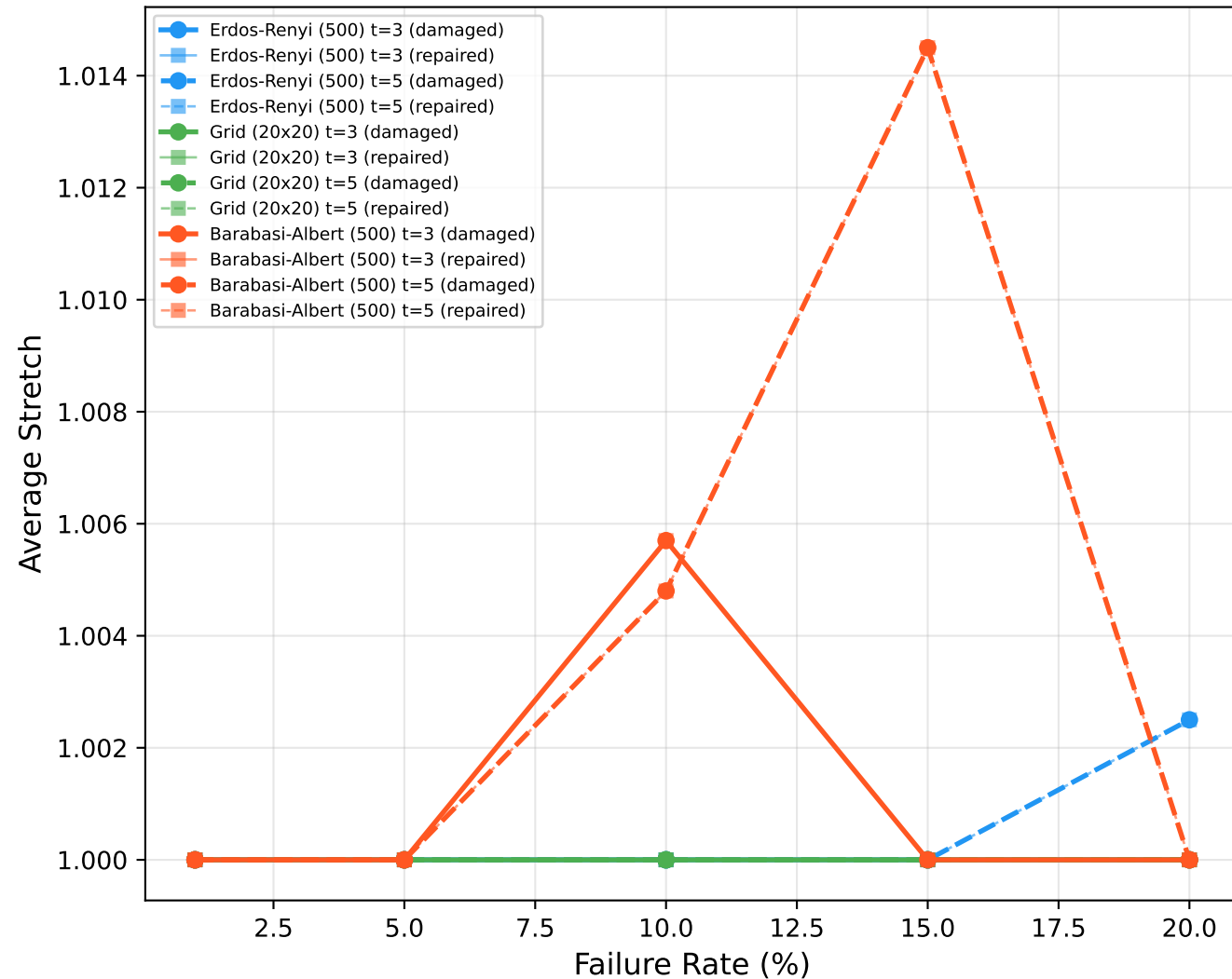
Stretch Degradation Under Node Failures
