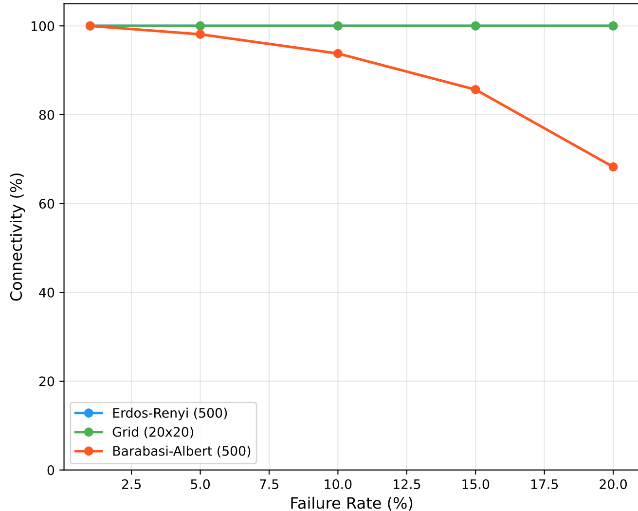
Spanner Connectivity Under Node Failures
