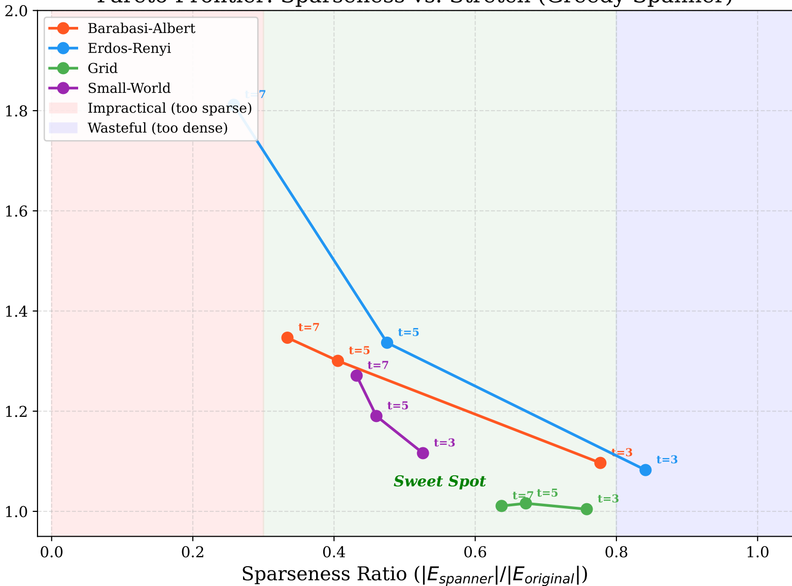
Pareto Frontier: Sparseness vs. Stretch (Greedy Spanner)
