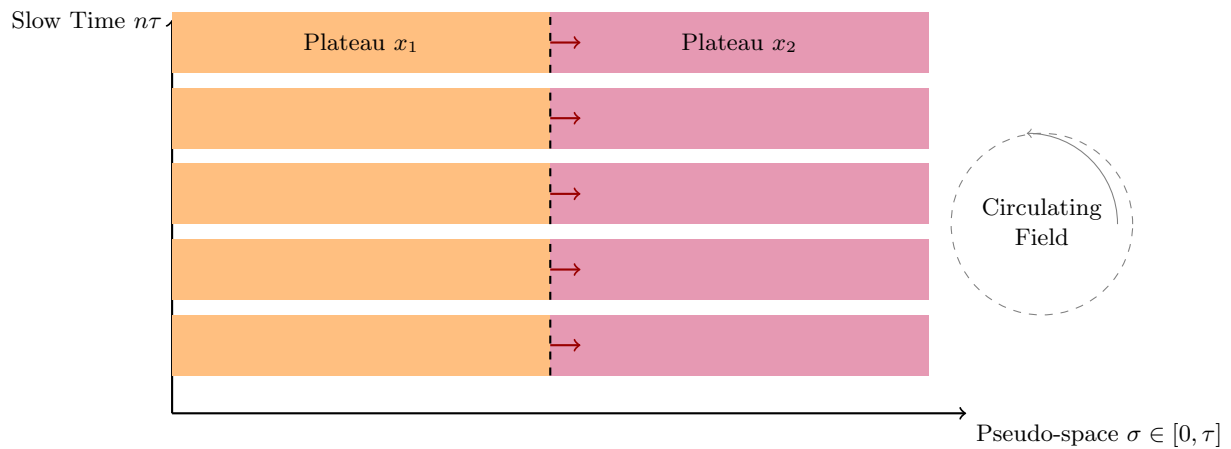
Delay-Induced Pattern Formation in Nonlinear Loops
