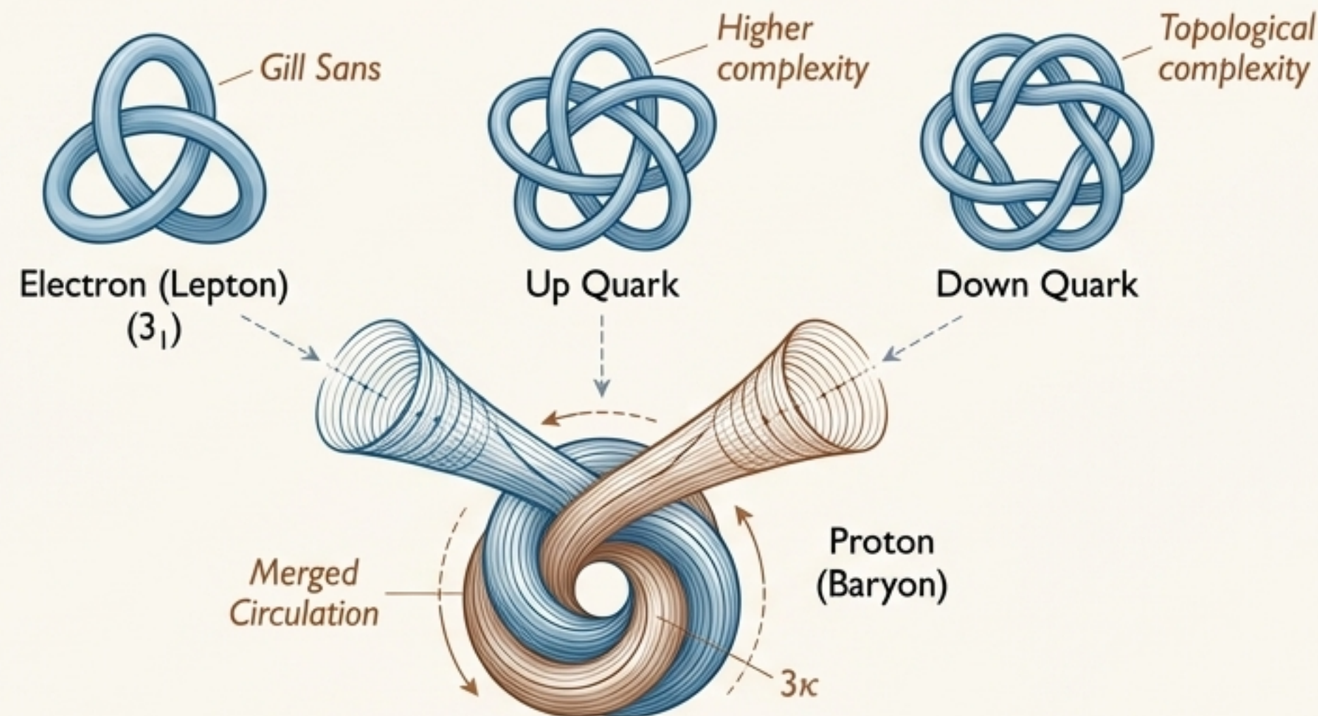
Knot-Particle Correspondence
