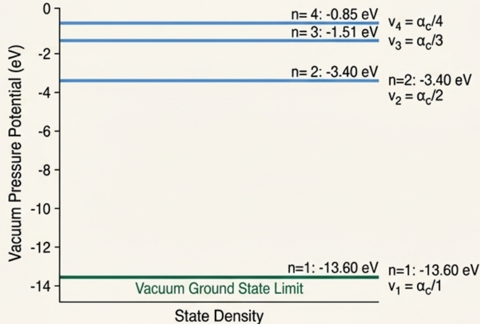
SST Hydrodynamic Energy Spectrum
