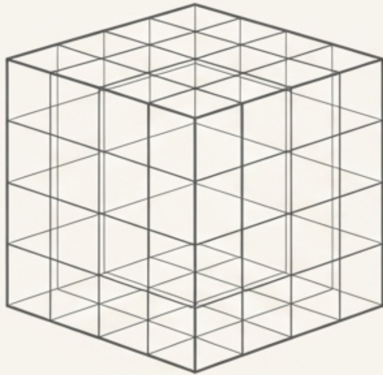
Empty, Geometric Vacuum
