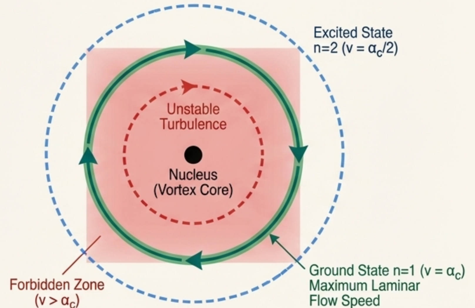
The Vacuum Stability Limit ( \alpha \approx 1/137 )
