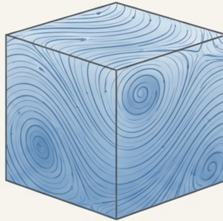
Frictionless Superfluid Medium
