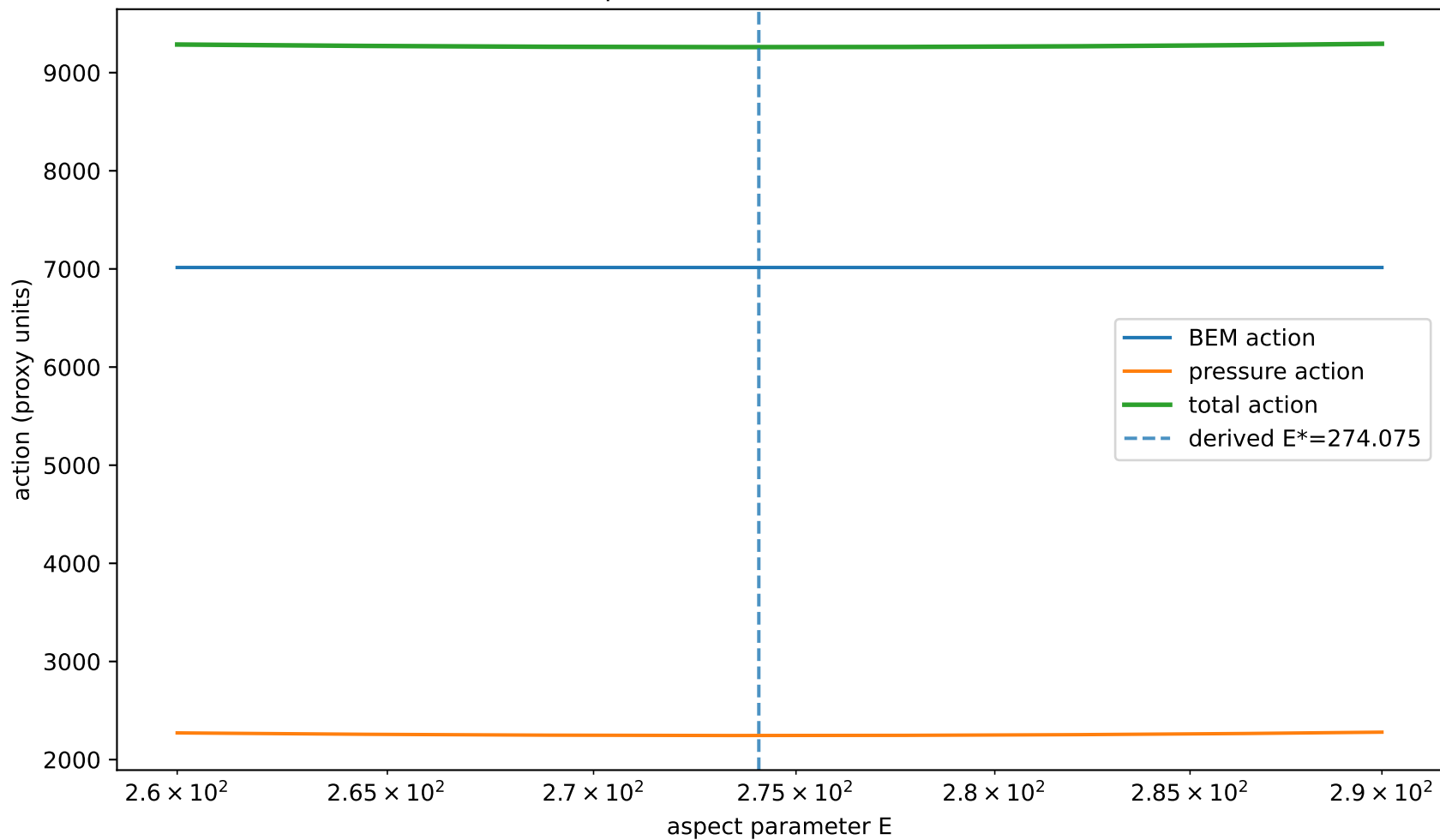
BEM/pressure finite-cell action scan
