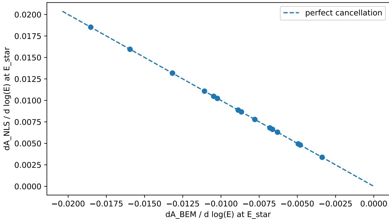
Stationarity as derivative cancellation
