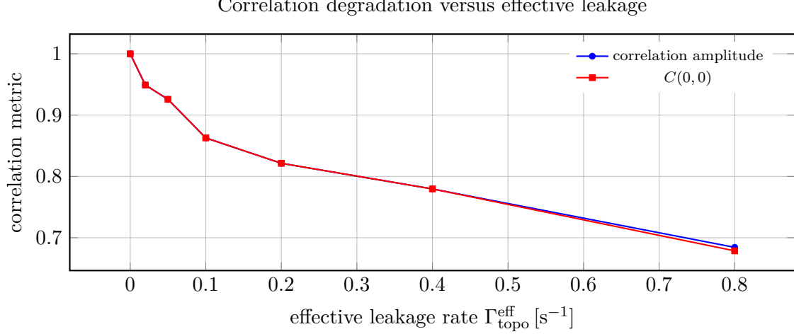
Figure 1: Correlation degradation under an effective leakage/decoherence surrogate. The plotted quantities are the correlation amplitude and the equal-analyzer value C(0,0) versus an effective leakage rate \Gamma_{\text{topo}}^{\text{eff}} in the reduced model. Although this leakage term is only a toy-model surrogate rather than a first-principles SST reconnection calculation, it makes explicit how finite phase memory degrades the reduced observable correlations.
