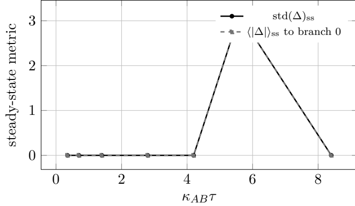
Figure 3: Steady-state locking diagnostics versus the control parameter \kappa_{AB}\tau , shown through the post-transient standard deviation \text{std}(\Delta)_{\text{ss}} and the mean branch distance to the in-phase branch, \langle|\Delta|\rangle_{\text{ss}} . This compact summary complements figure 2 by showing how the delayed branch locking changes across the sampled sweep.
