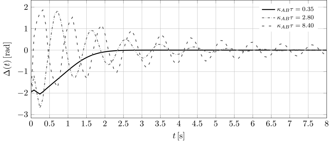
Representative time series across the locking sweep
