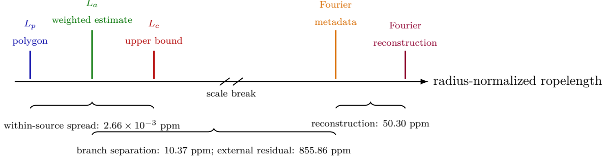
FIG. 4. Provenance hierarchy for the high-resolution and Fourier branches. The horizontal scale is deliberately broken between the high-resolution cluster and the Fourier points. The weighted value L_a is an estimate, whereas L_c is the reported inscribed-curve upper bound. The reconstruction point is obtained by re-deriving the centerline length from the stored Fourier coefficients; its separation from the metadata value is roughly five times the metadata–high-resolution branch separation, and still more than an order of magnitude below the external residual.
