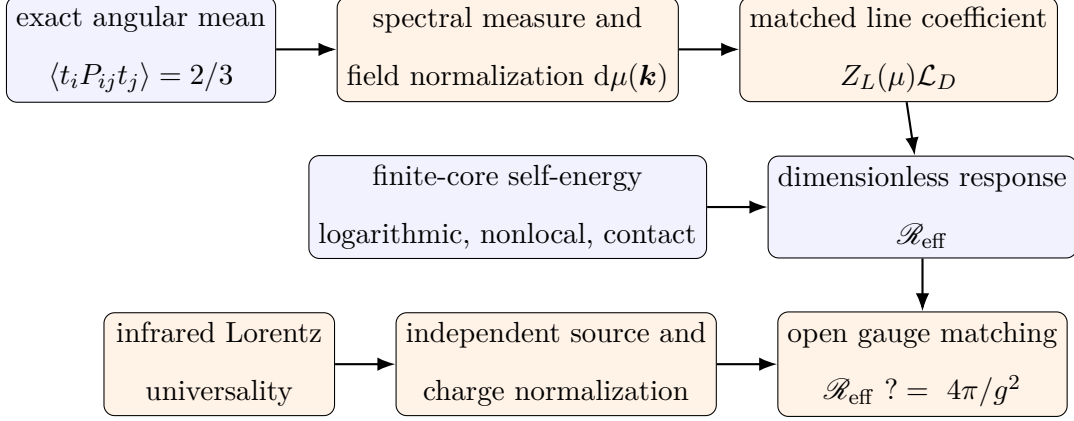
FIG. 2. Logical separation of the exact normalized angular identity, the open spectral-measure normalization, finite-core energy, source normalization, Lorentz universality, and the optional gauge-stiffness interpretation. The value 8\pi/3 corresponds to one unnormalized angular convention; it is not fixed by transversality alone.
