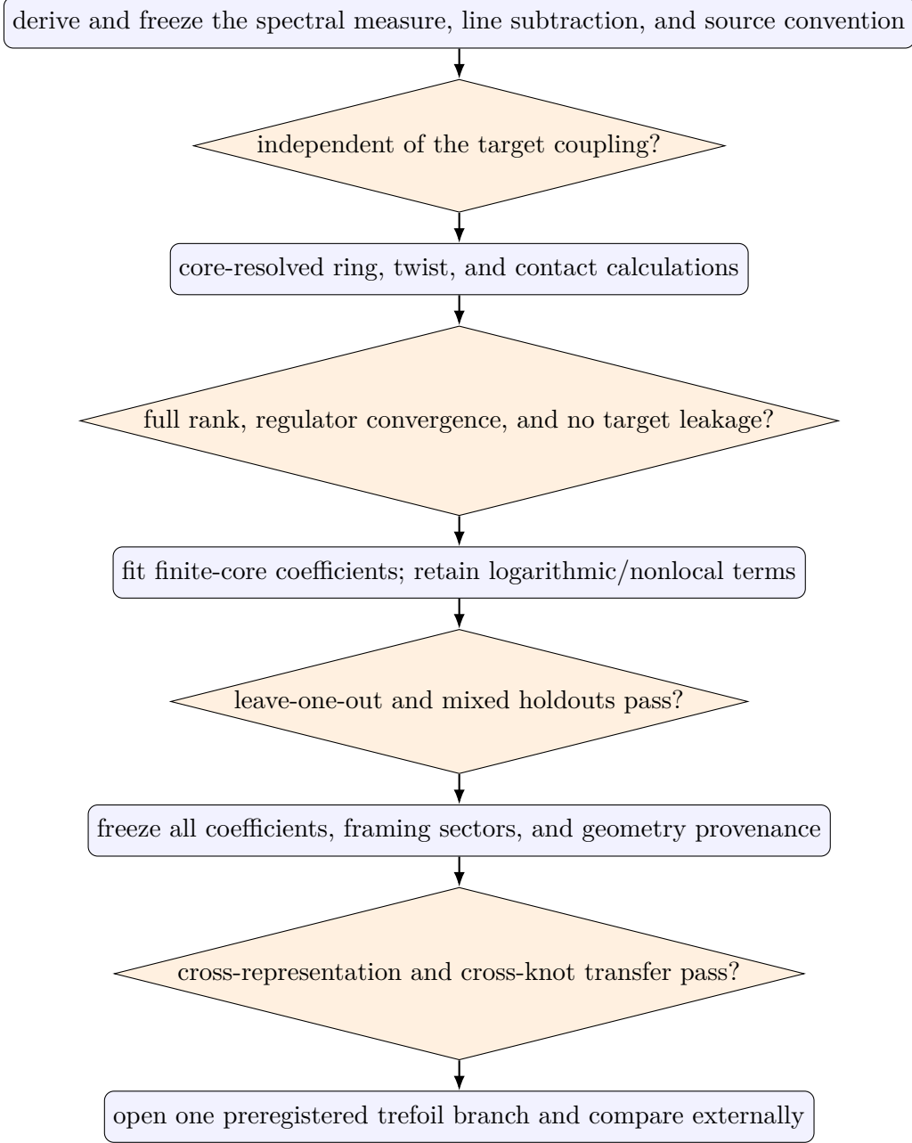
FIG. 5. Revised calibration and falsification sequence. The normalization of the leading length term is itself part of the independent matching problem; it is not supplied by the angular identity.
