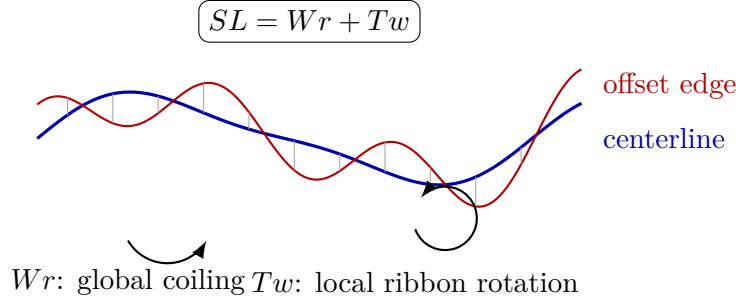
FIG. 3. Schematic ribbon representation of self-linking. Writhe is a nonlocal property of the centerline, while twist requires a chosen material framing. The drawing is illustrative rather than a numerical trefoil reconstruction.
