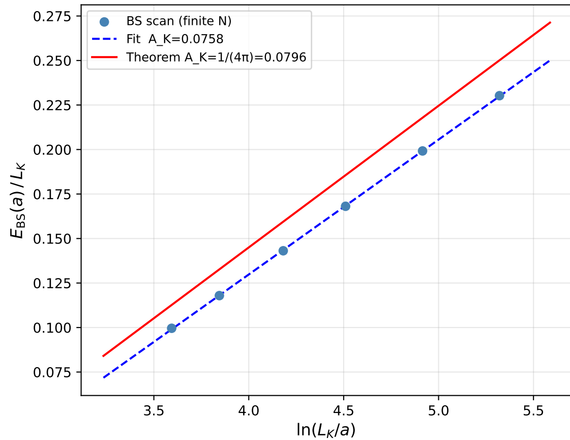
Trefoil Biot-Savart log coefficient
