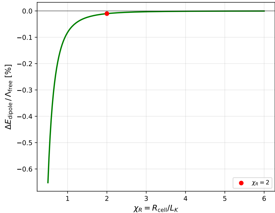
Neumann dipole correction fraction
