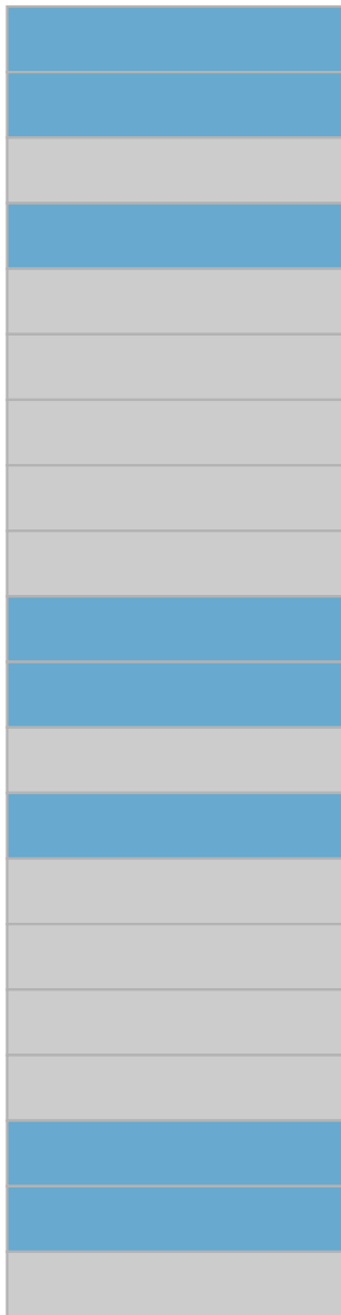
WHO 3/3
