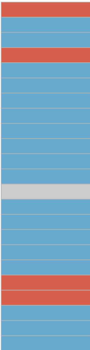
WHO 2/3
