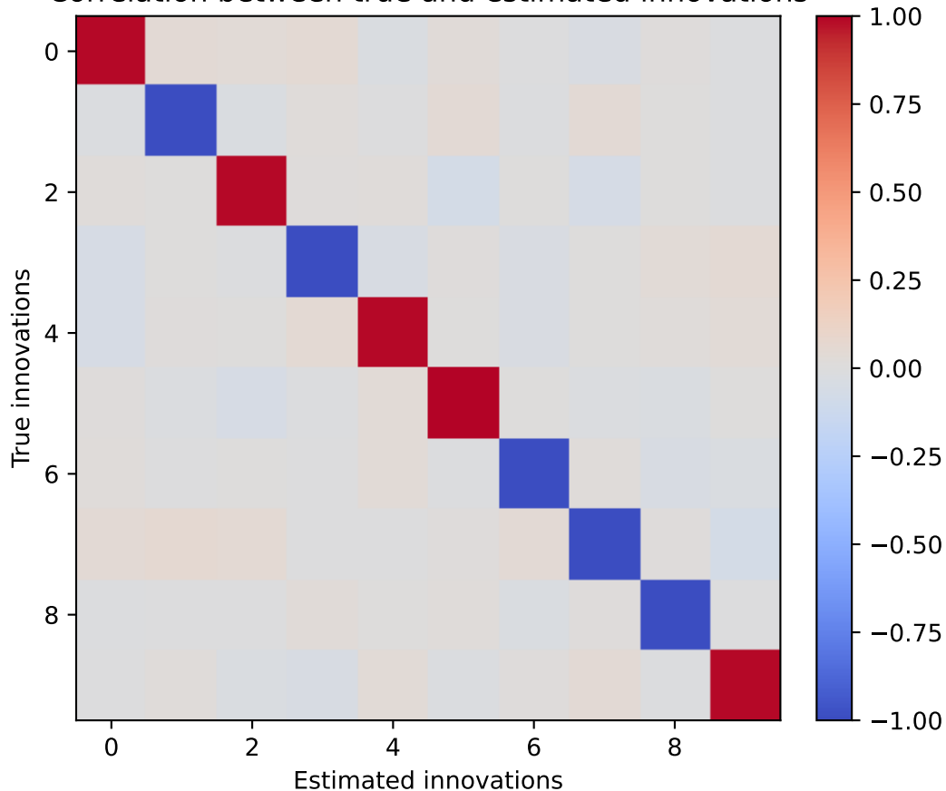
Correlation between true and estimated innovations
