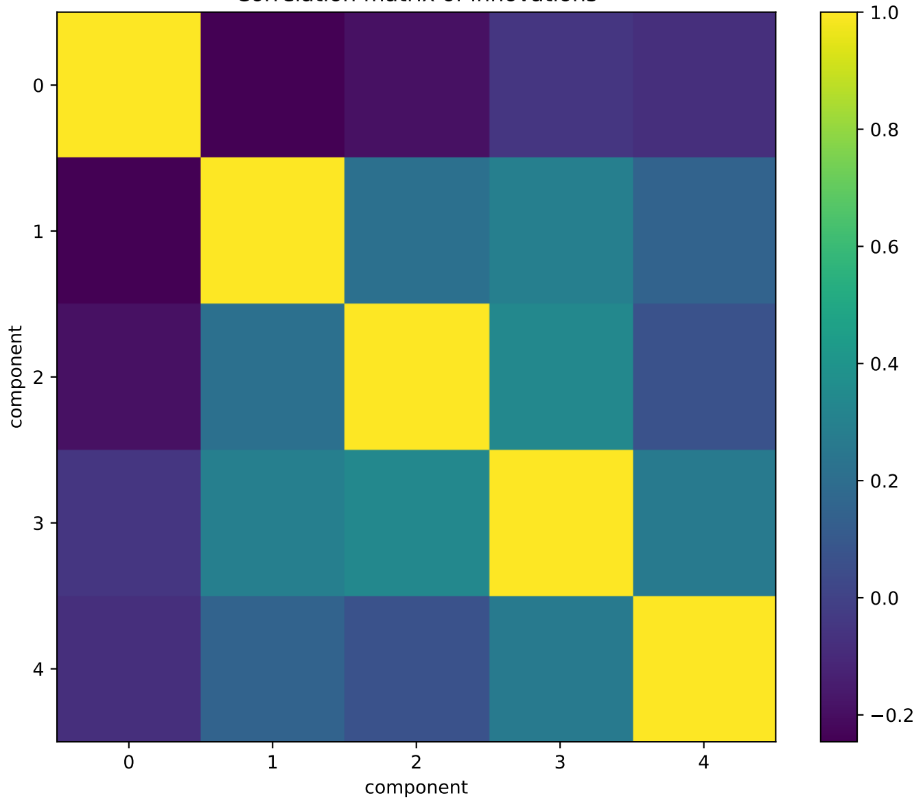
Correlation matrix of innovations
