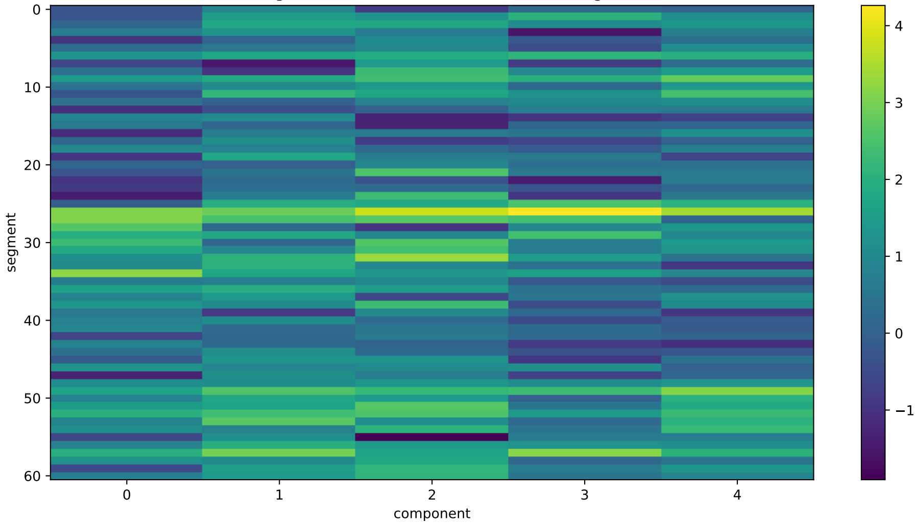
Segment-wise variance of innovations (log)
