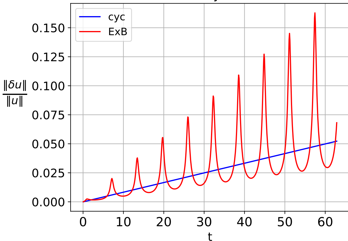
Relative velocity error in time
