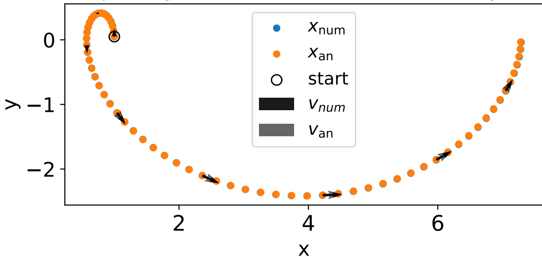
Trajectory of ExB drift (numeric vs analytic)
