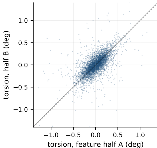
Reference-anchored r = 0.623 , reliability = 0.768
