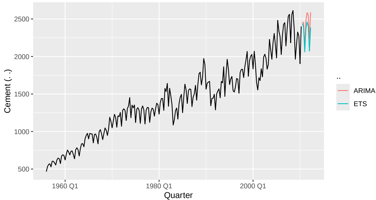
ARIMA vs ETS .. .. (Cement)
