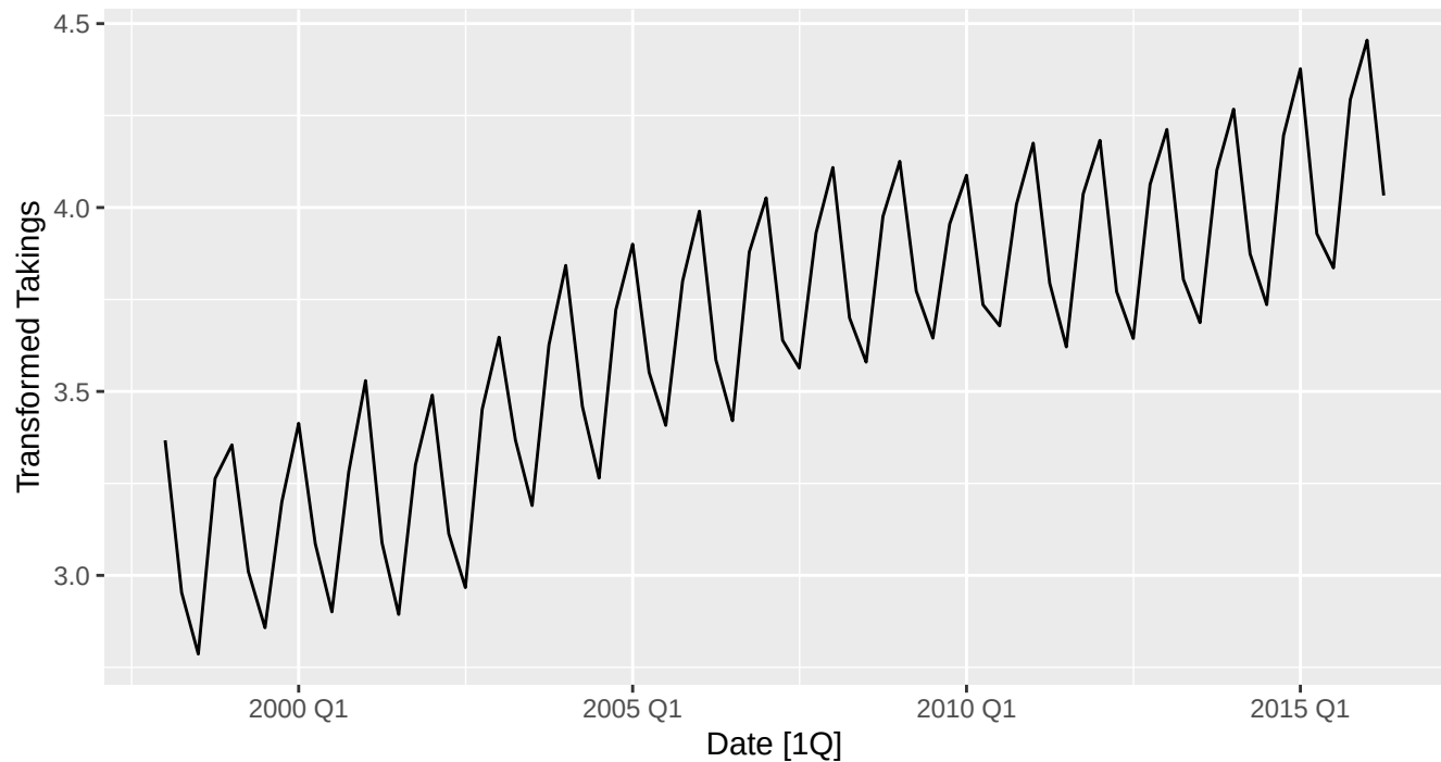
Box-Cox ... Tasmania Takings (lambda = 0.002)
